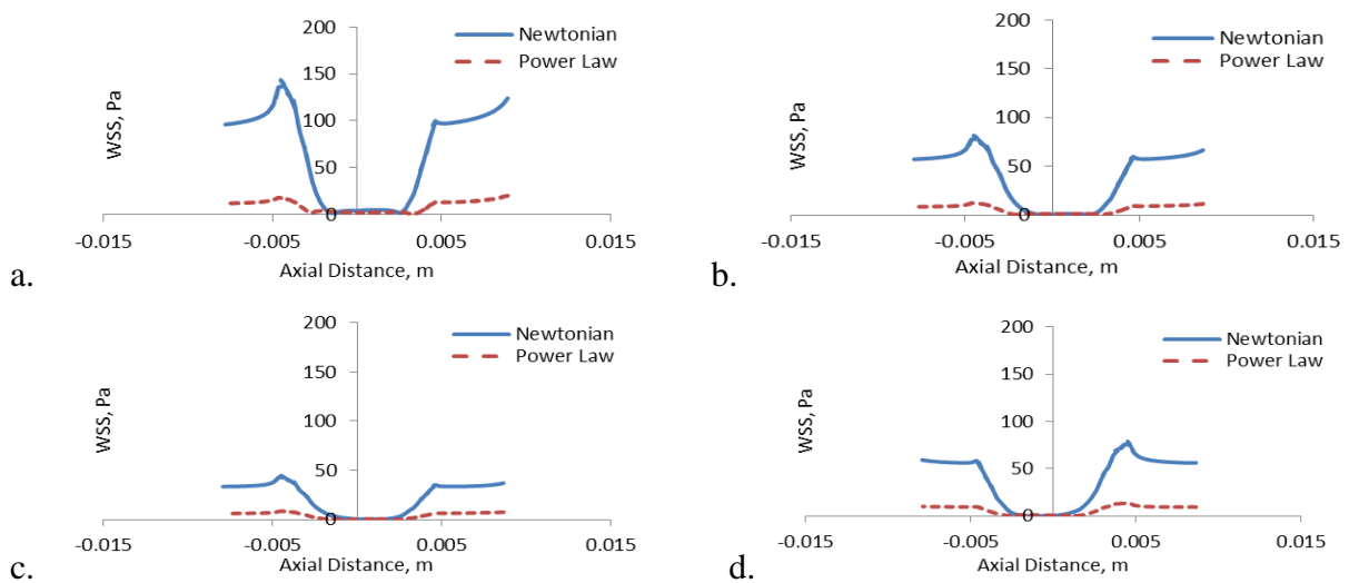
Fig. 6 WSS in axial z-direction at time interval, a. t=0.25s , b. t=0.50s , c. t=0.75s , d. t=1.0s
