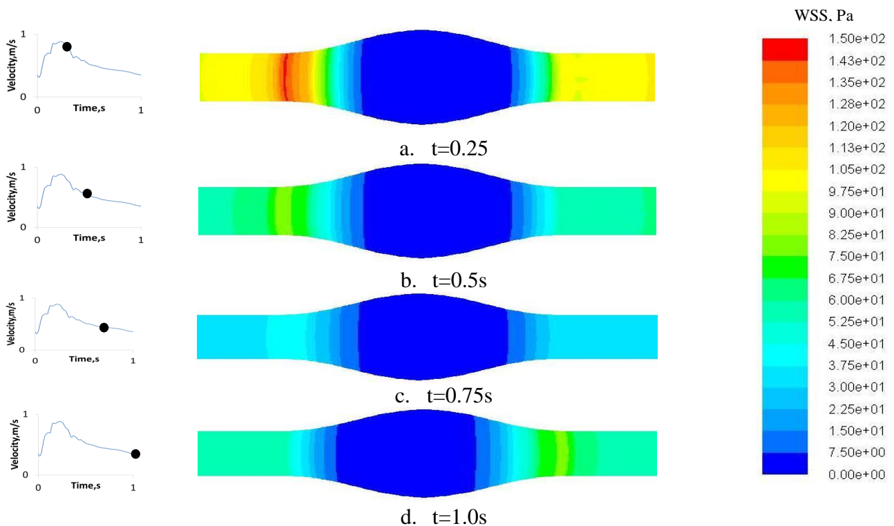
Fig. 4 Wall Shear Stress Contour for Newtonian model
