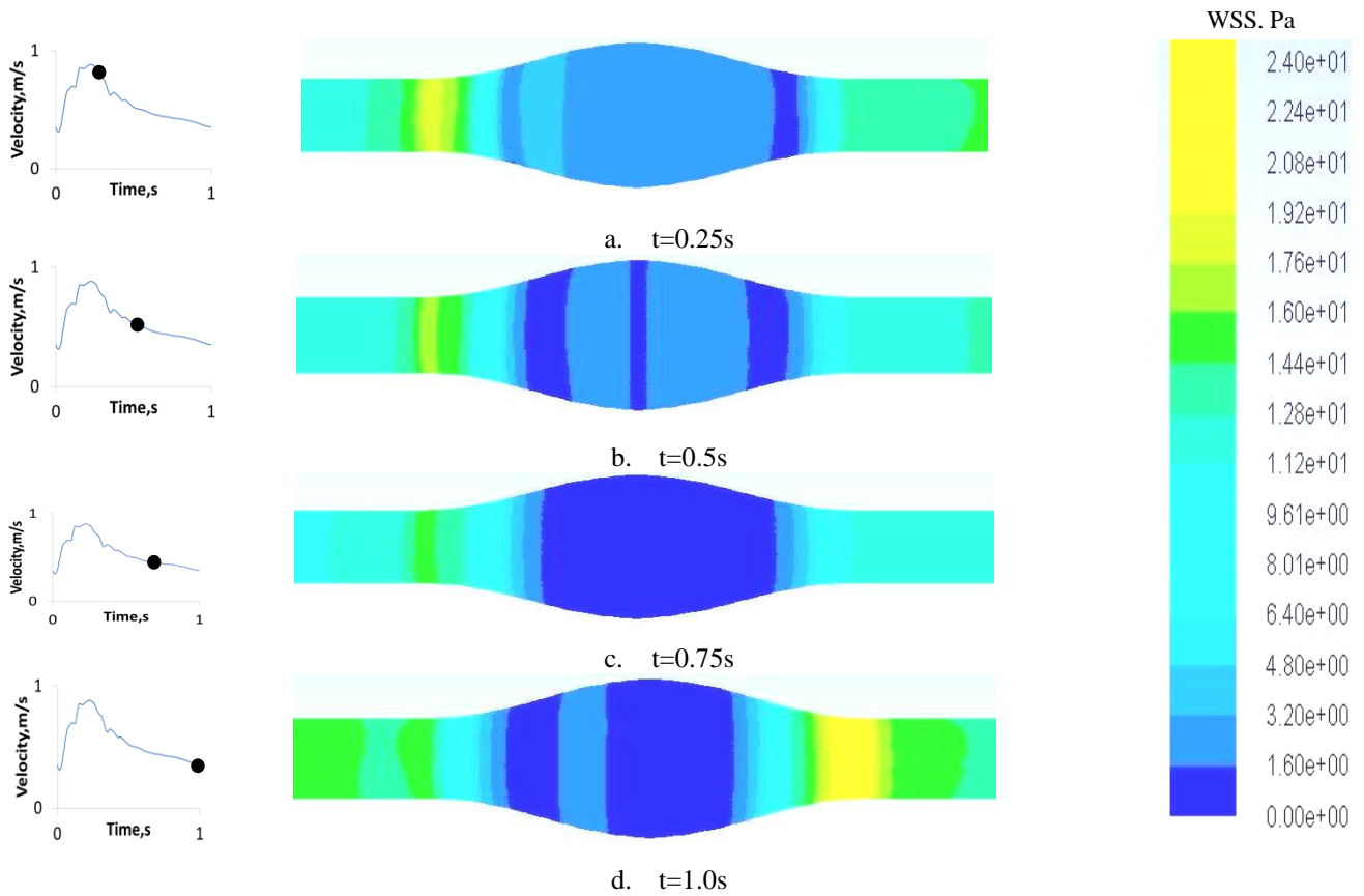
Fig. 5 Wall Shear Stress Contour for Power Law model
